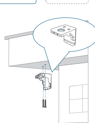
Ceiling Mounting
