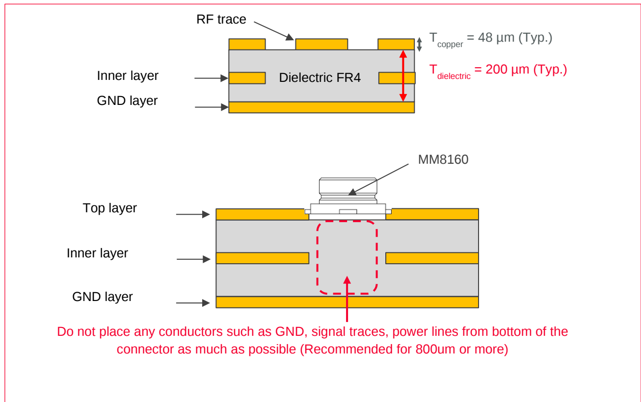
Figure 5: PCB Stack-Up Layers
