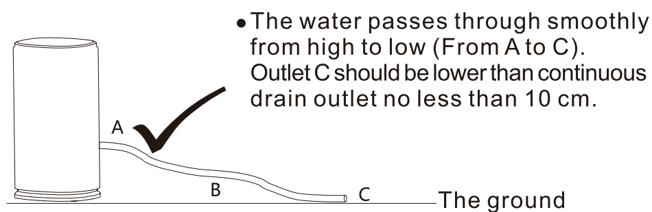
Picture 3: Example of a correct connection
