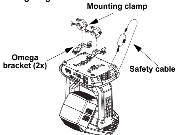
Overhead mounting
