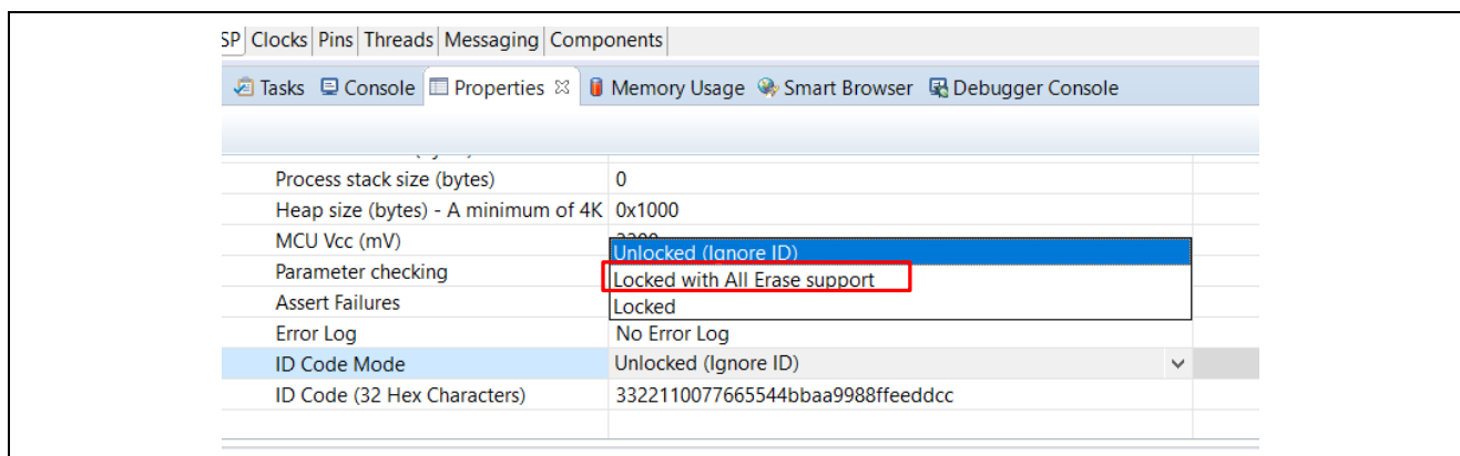
Figure 13. Setting up OSIS ID using RA MCU Configurator
