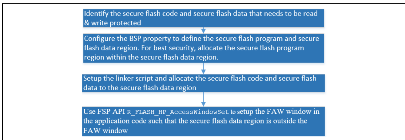
Figure 17. Establish Read/write Protected Internal Flash Region
