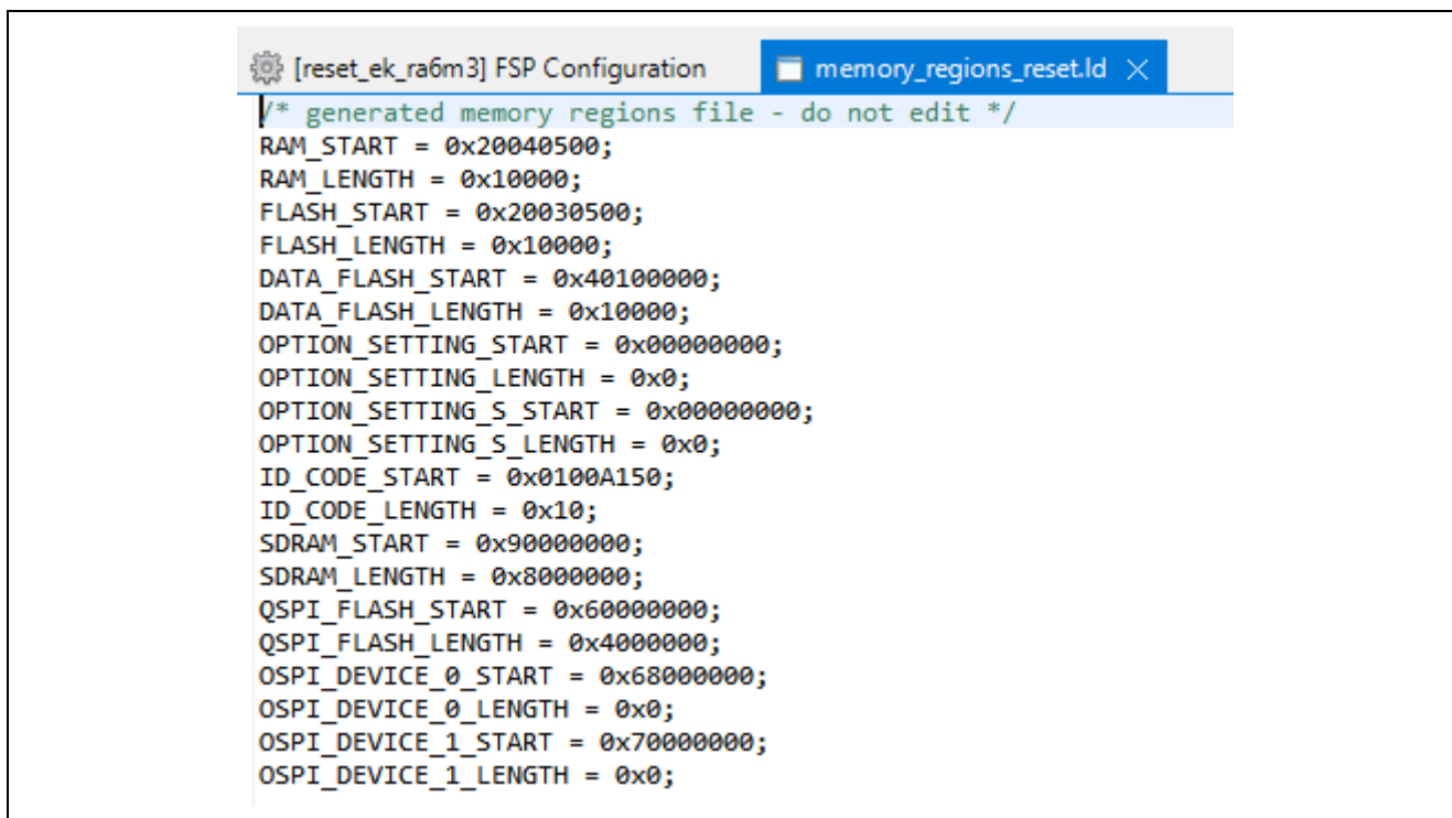
Figure 44. Customized Linker Script for reset_ek_ra6m3 Project
