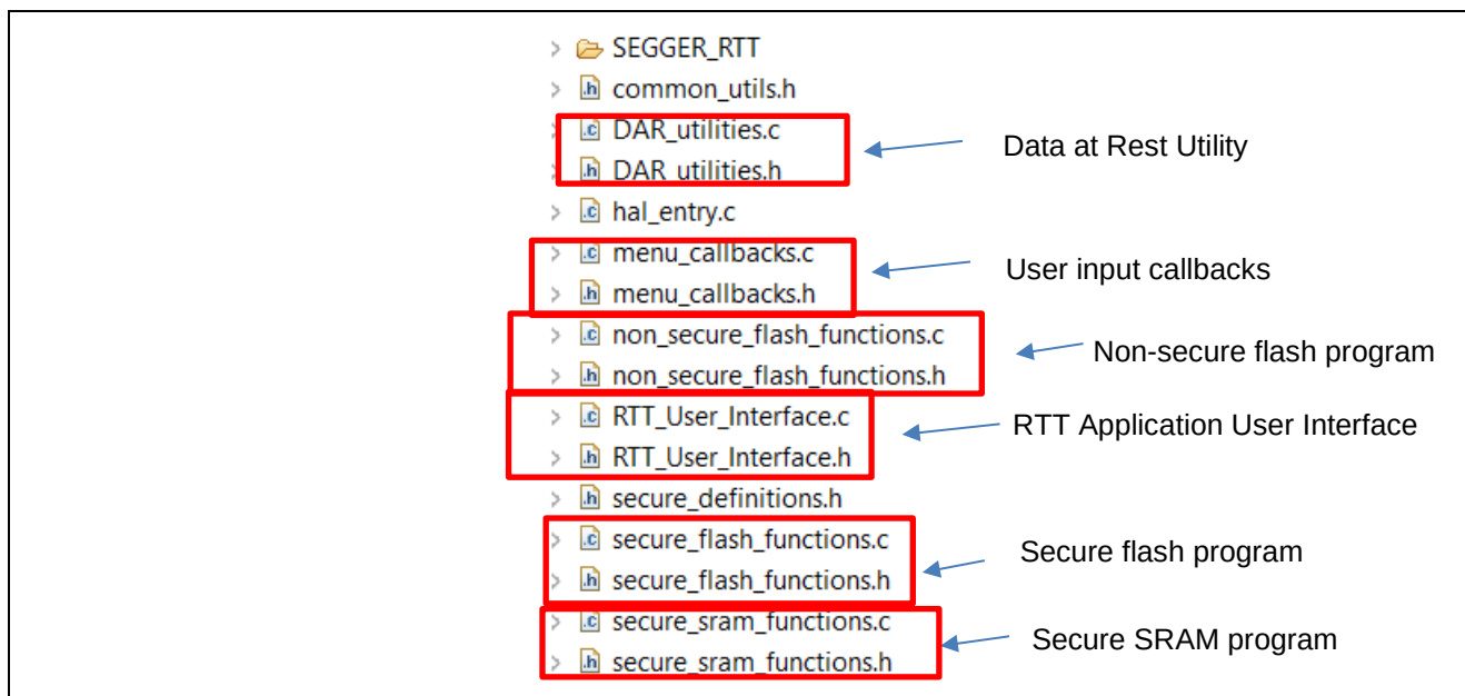
Figure 23. Source Code
