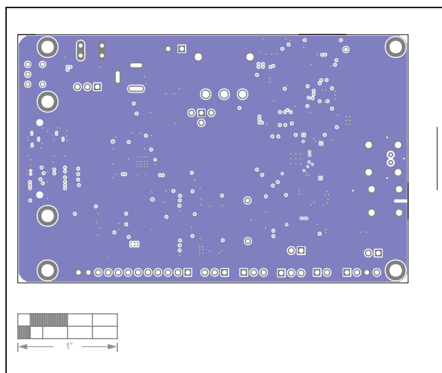
MAX96717 EV Kit—Layer7
