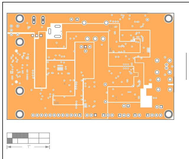
MAX96717 EV Kit—Layer5
