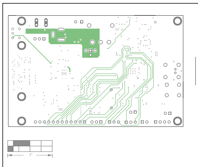
MAX96717 EV Kit—Layer3
