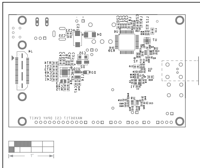
MAX96717 EV Kit—Silk Bottom
