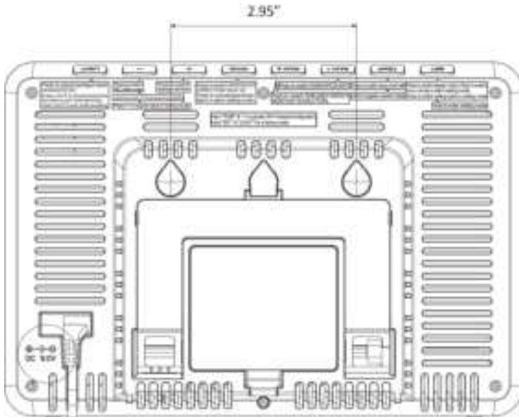
Figure 21: Rear view (Refer to 3.4 for Button functions)
