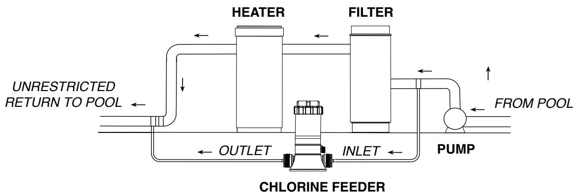
FIGURE INSTALLATION & PIPING LAYOUT
