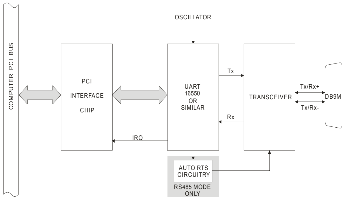
Figure 1-1: Block Diagram
