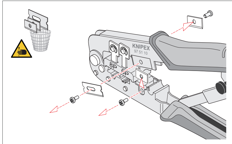
Changing blades
