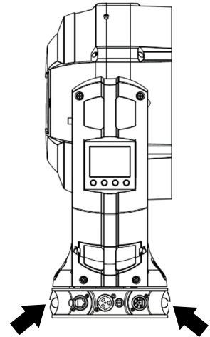
Figure 2. Safety cable attachment points
