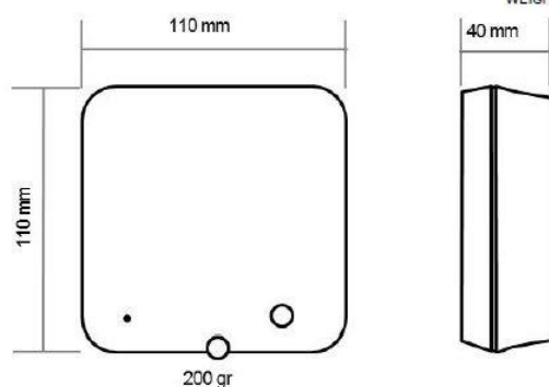
RECEIVER BOX
