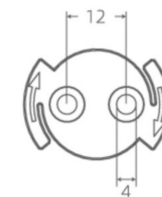
Mounting board size: 22.4 x 29.6 x 4.7
