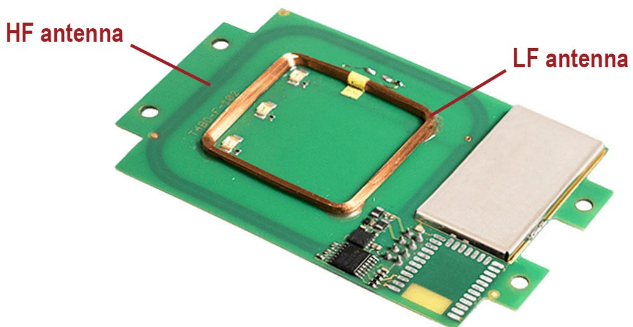
PCB contained in TWN4 MultiTech 2 LF HF
