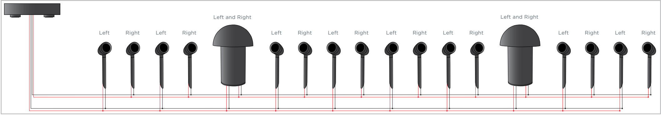
SONARRAY 16:2 CONFIGURATION
