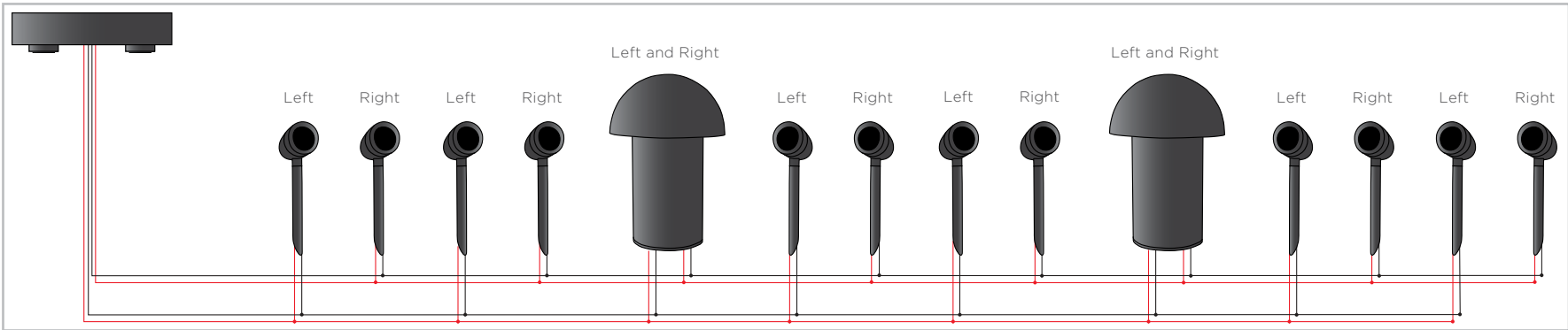
SONARRAY 12:2 CONFIGURATION
