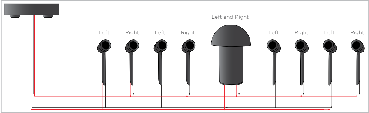
SONARRAY 8:1 CONFIGURATION
