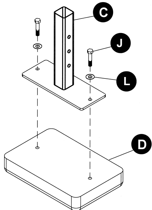
SEAT ASSEMBLY
