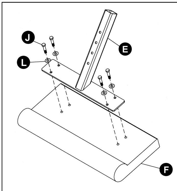
ARMREST ASSEMBLY
