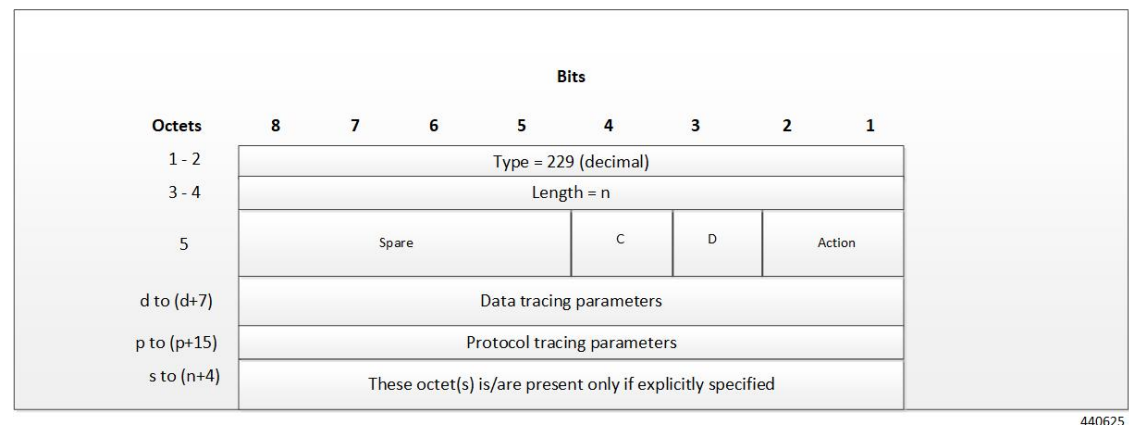
Figure 18: Subscriber Tracing
