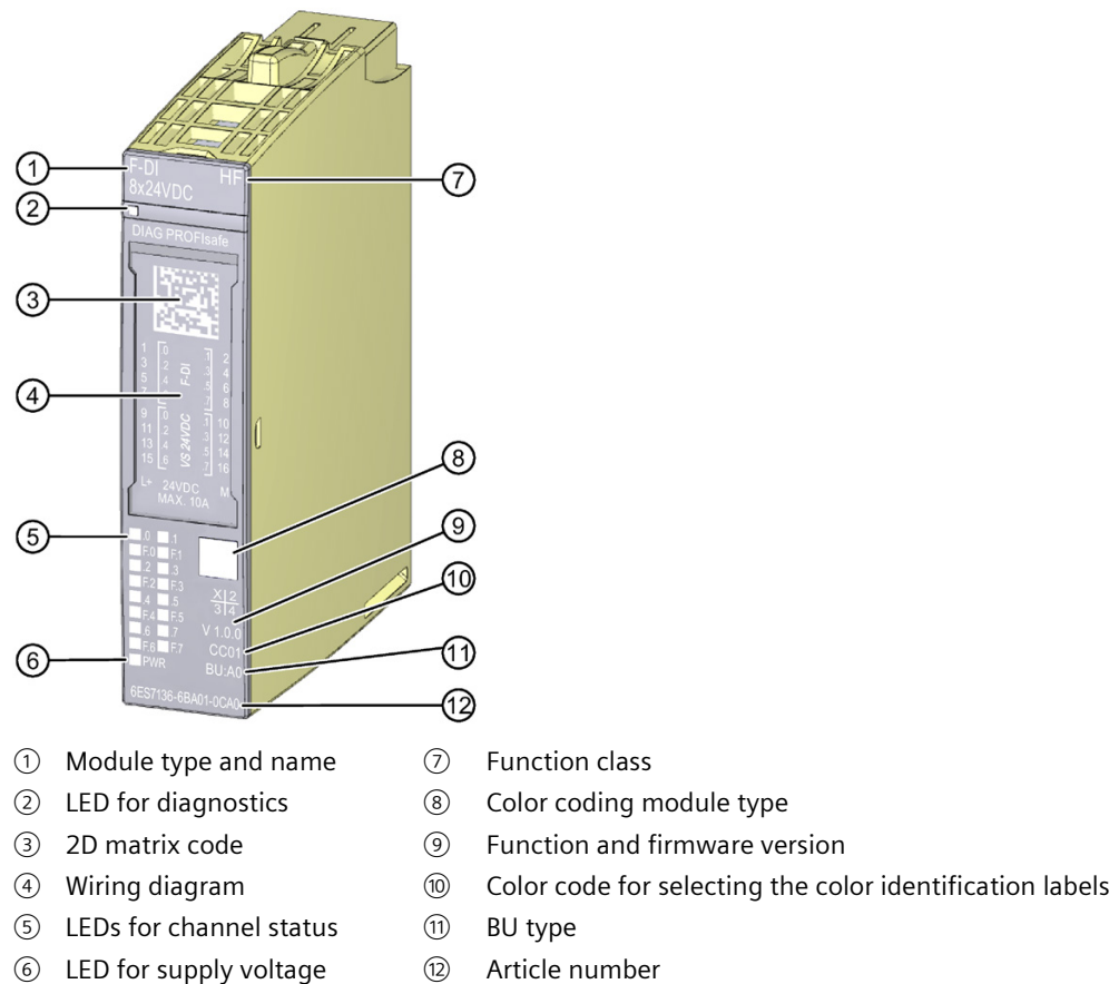
Figure 2-1 View of the F-DI 8x24VDC HF module
