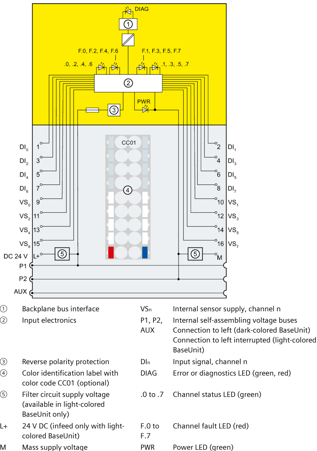
Figure 3-1 Block diagram
