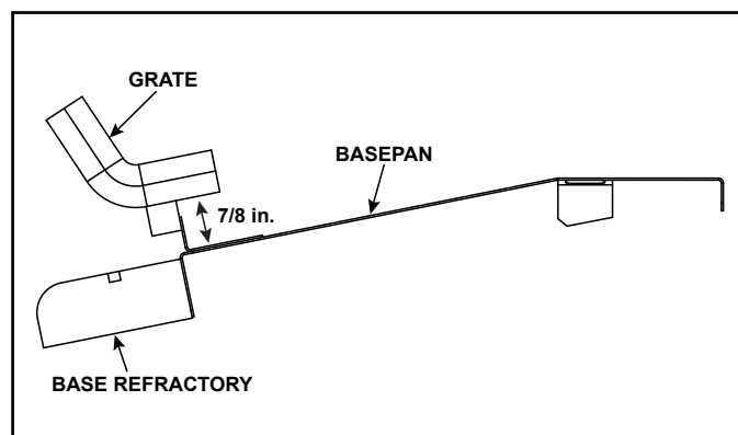
Figure 27. Side Profile Grate Location Reference
