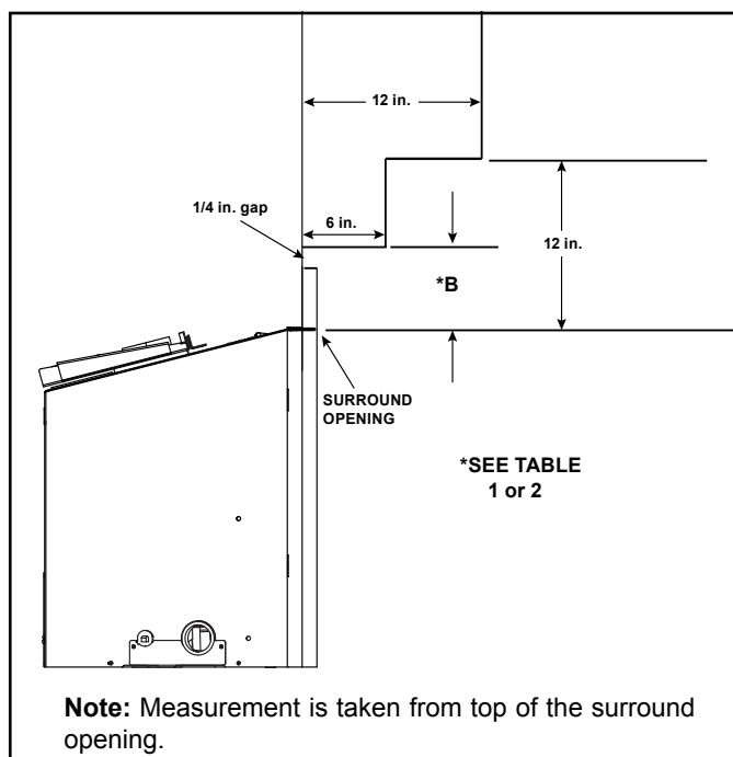
Figure 3.16 Minimum Vertical and Maximum Horizontal Dimensions - Non-Combustible
