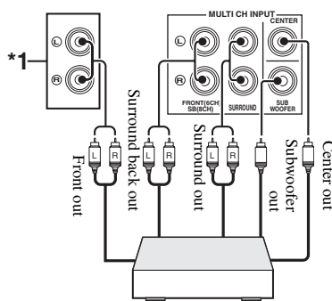
Multi-format player/External decoder (7.1-channel output)
