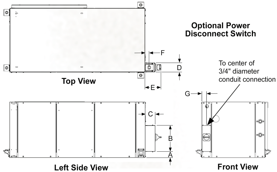
Figure 21: Optional Non-Fused Disconnect Switch Location and Dimensions
