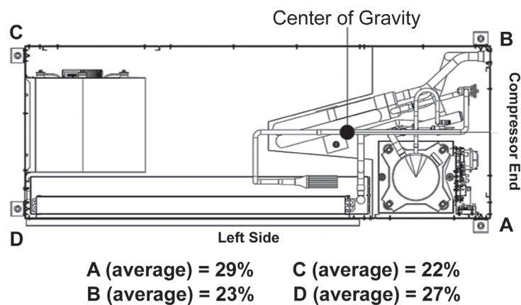
Figure 1: Horizontal Unit Corner Weights - Letter Reference for Table 4
