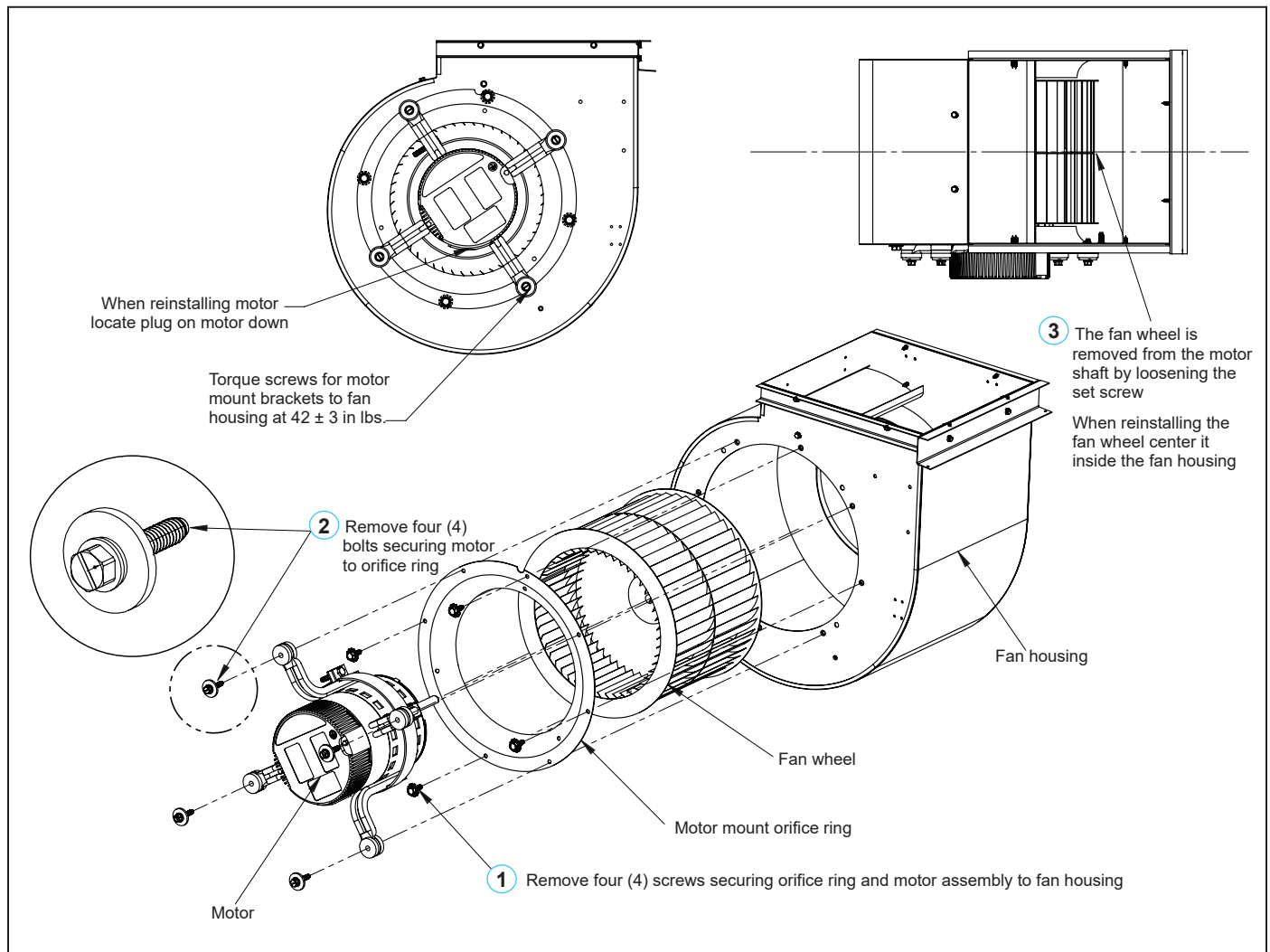
Figure 40: Disassemble Motor Orifice Ring and Motor Mount Screws From Fan Housing
