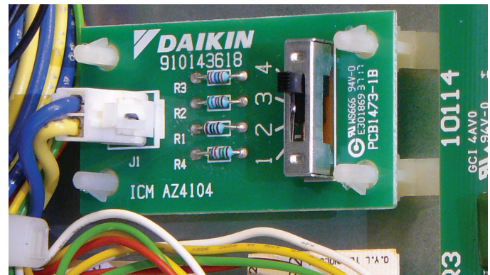
Figure 38: 4-Position Fan Speed Selector Switch
