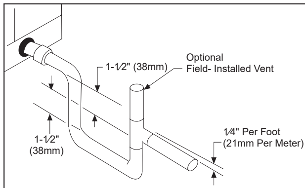
Figure 30: Unit Condensate Drain Pipe Trap Detail
