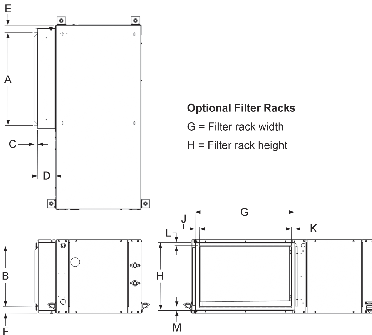
Figure 15: Filter Rack, Return Duct Collar Dimensions
