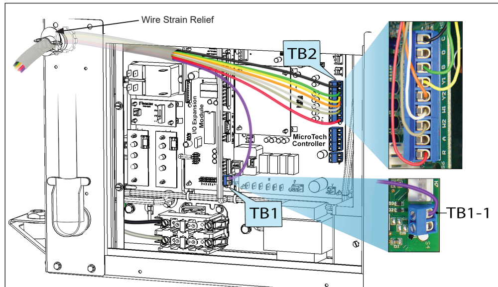
Figure 23: Terminal Connections To TB2 (Thermostat Control) On The MTIII Board
