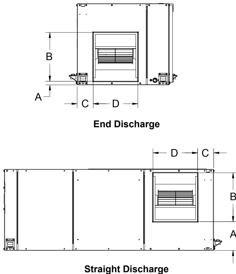
Figure 16: GCH Discharge Air Duct Collars Locations and Dimensions
