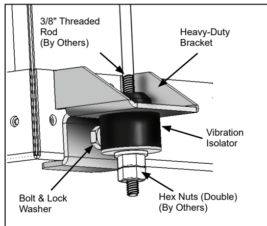
Figure 2: Heavy-duty hanger brackets (sizes 060-070)
