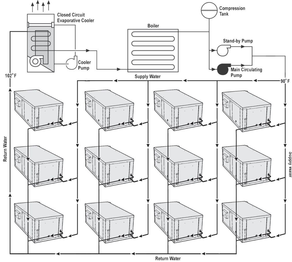
Figure 7: Example of A Reverse Return Piping System
