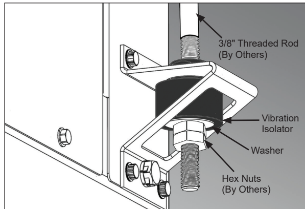
Figure 8: Hanger Bracket Detail - Sizes 007 Through 070
