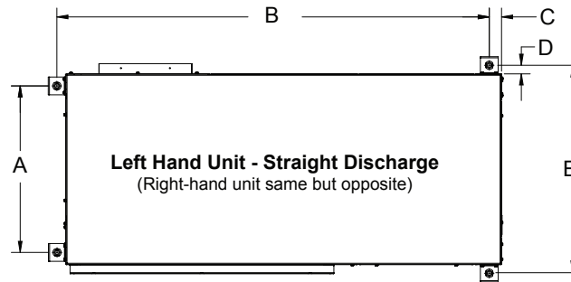
Figure 9: Hanger Bracket Locations Dimensions - Sizes 007 Through 070
