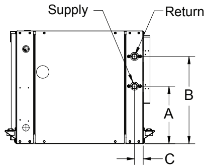
Front View - Water Connections
