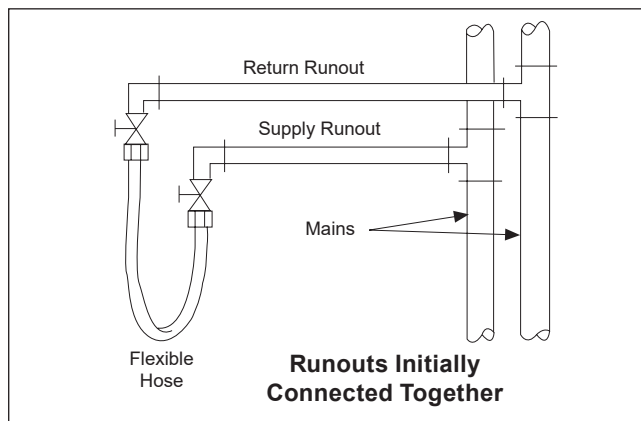
Figure 31: Supply and Return Runouts Connected Together
