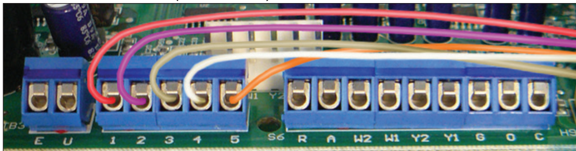
Figure 25: Terminal Connections To TB1 (Sensor Control) On The MTIII Board
