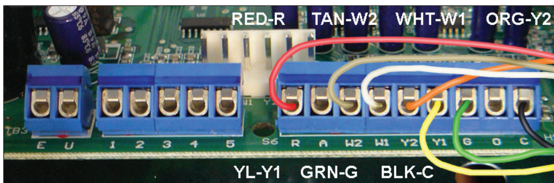
Figure 24: Terminal Connections To TB2 (Thermostat Control) On The MTIII Board
