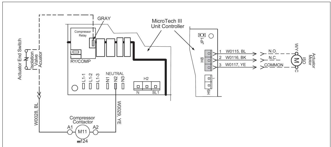
Figure 39: Motorized Valve Wiring
