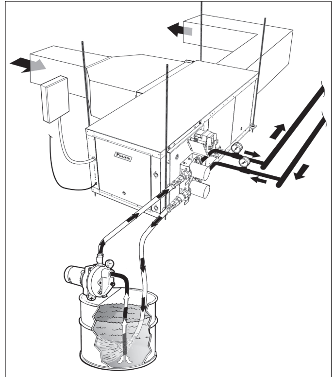
Figure 4: Flushing The Loop
