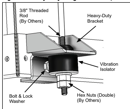
Figure 2: Heavy-duty hanger brackets (sizes 042-048)
