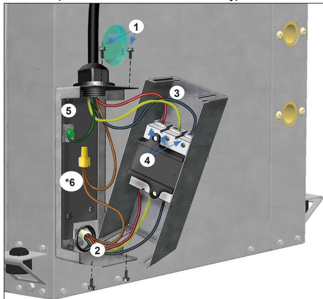
Figure 22: 460V Wiring With Neutral Wire (*Constant CFM EC Motors Only) To The Non-Fused Disconnect Switch
