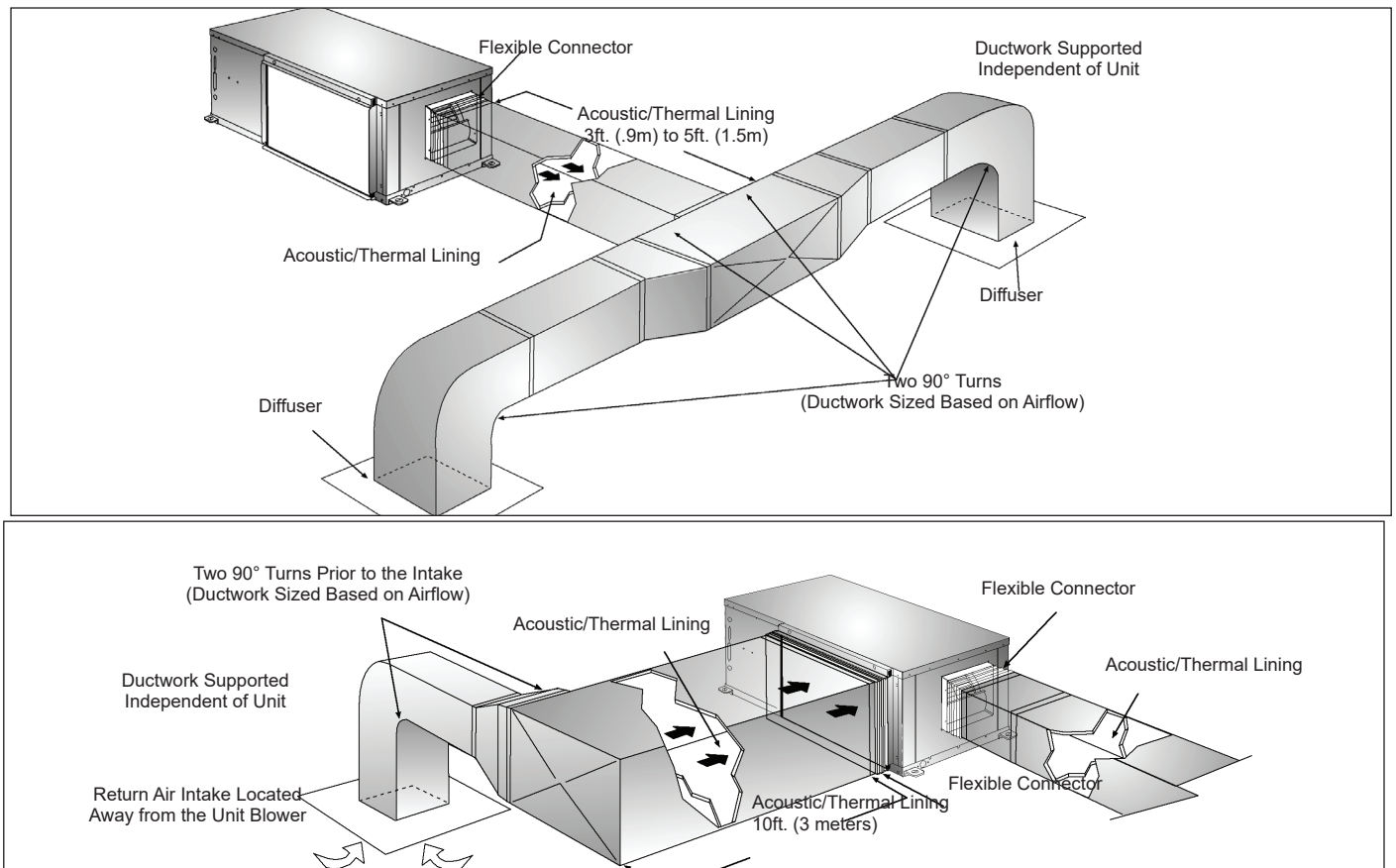
Figure 14: Typical Ducting for Horizontal Unit
