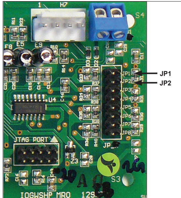
Figure 37: JP1 & JP2 Location On The I/O Expansion Module
