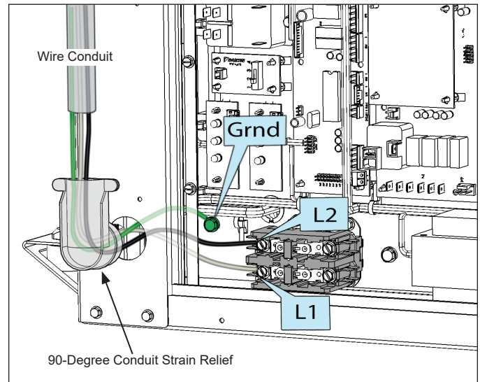
Figure 20: Line Voltage Wiring Route To Wire Connections
