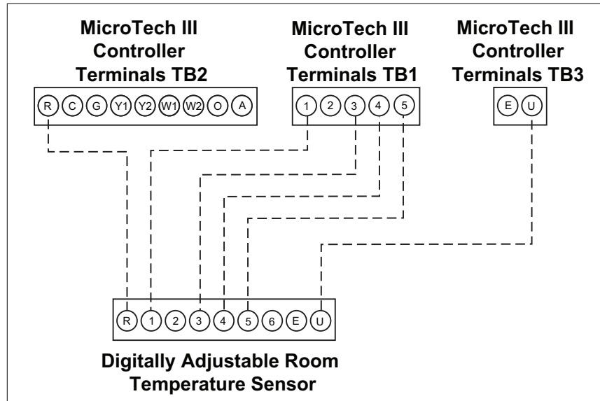
Figure 27: Digitally Adjustable Room Temperature Sensor Wiring
