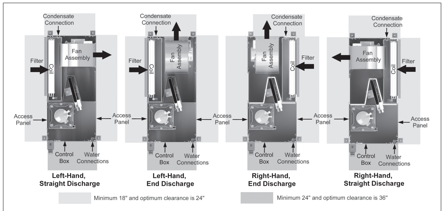
Figure 11: Recommended Clearances for Service Access
