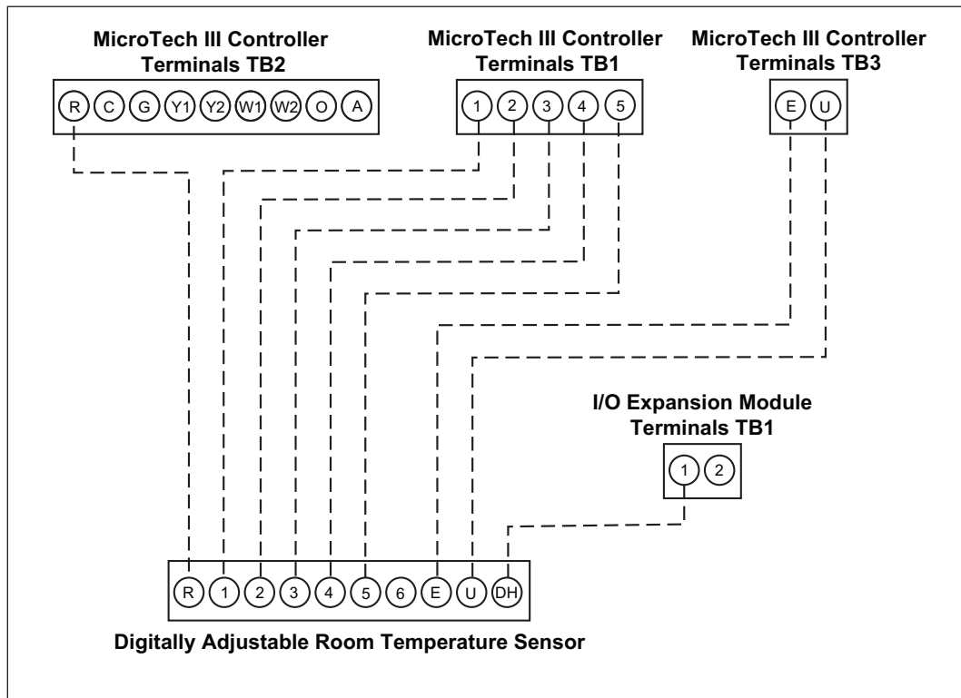
Figure 28: Digitally Adjustable Room Temperature and Humidity Sensor Wiring
