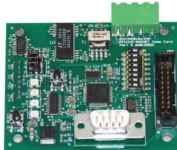
Figure 35: MicroTech III BACnet Water Source Heat Pump Snap-In Communication Module
