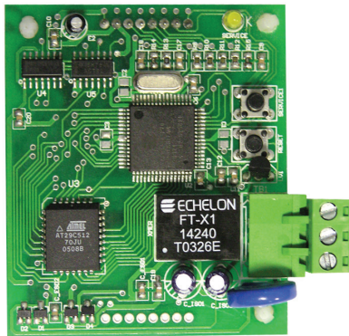
Figure 34: LONWORKS Communication Module
