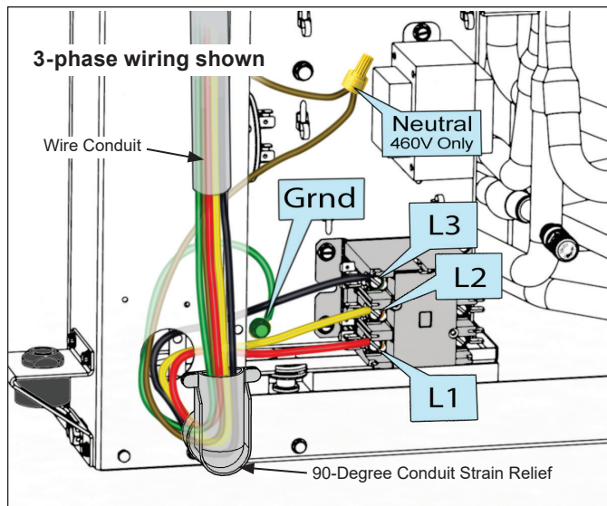
Figure 19: Route Line Voltage Wires To Terminal Screws
