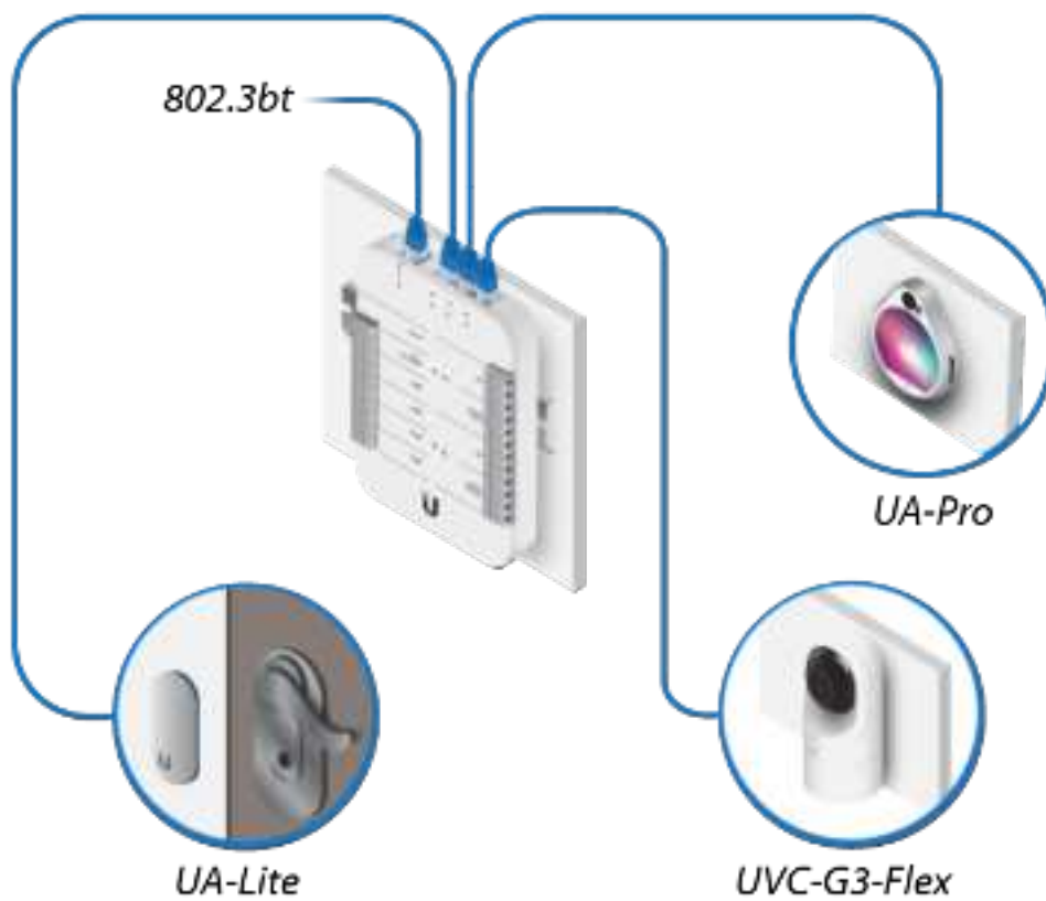
Sample UniFi Access Diagram
