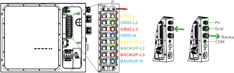
Terminal Layout
