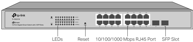
Figure 1-1 Front Panel of TL-SG2218
