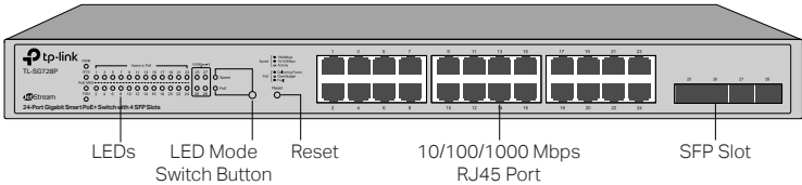
Figure 1-6 Front Panel of TL-SG728P
