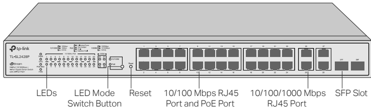
Figure 1-5 Front Panel of TL-SL2428P
