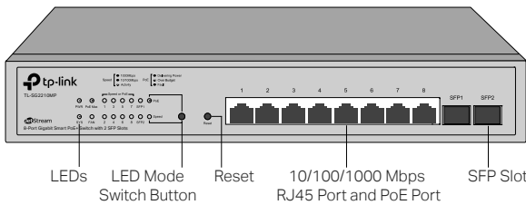
Figure 1-2 Front Panel of TL-SG2210MP
