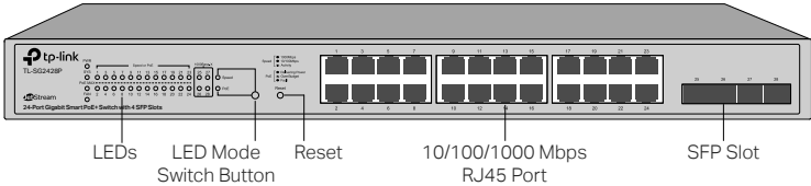
Figure 1-4 Front Panel of TL-SG2428P
