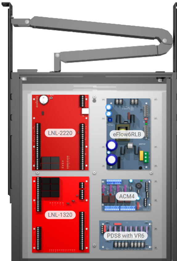
T1RM3F4 4-Door Rack Access System with Power
