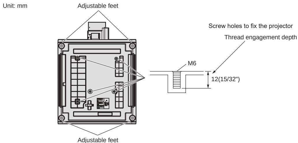
Positions of screw holes to fix projector and adjustable feet
