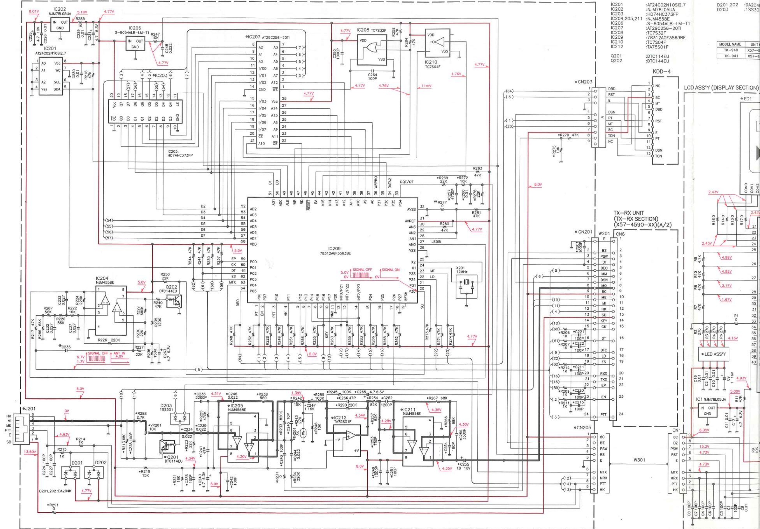
TX-RX UNIT (CONTROL SECTION) (X57-4590-XX)(B/2)
