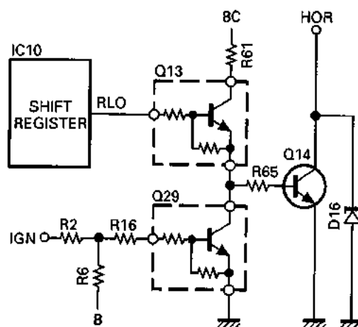
Fig. 8 Horn control circuit
