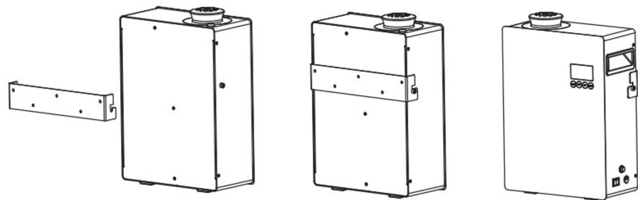
(Diagram of Wall-mounted Installation)
