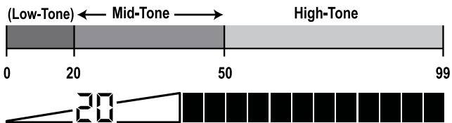
IRON AUDIO ON: Targets below 20 are now heard as a low tone and targets above 20 will produce a mid or high tone.
