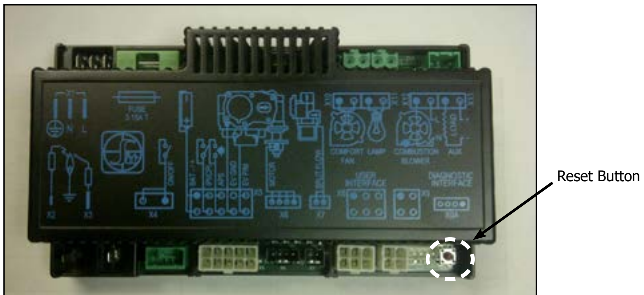
Figure 6: Integrated Fireplace Controller
