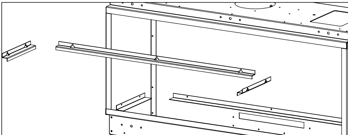
Figure 74: Panel Installation
