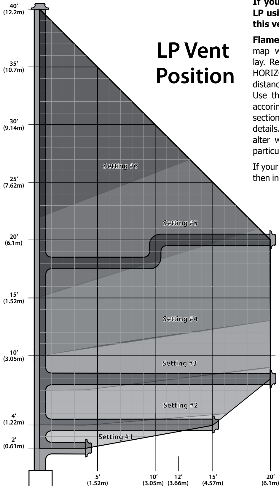
Figure 58: LP Vent Graph
