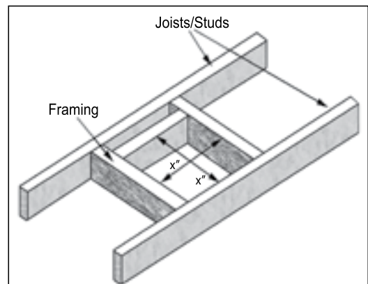
Figure 56: Vent Framing For Wall or Ceiling
