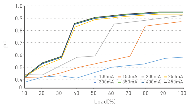
Power Factor Characteristic Curve
