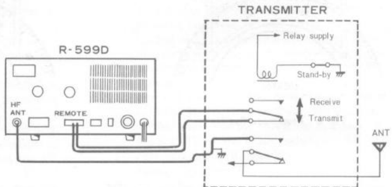
(b) Connection of Transmitter
