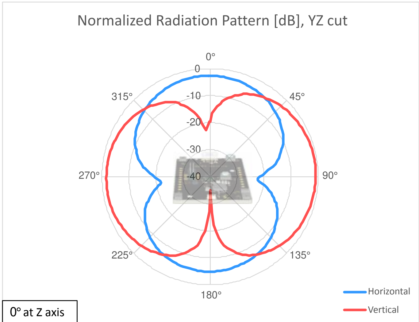
Figure 5.6. Antenna Pattern - YZ
