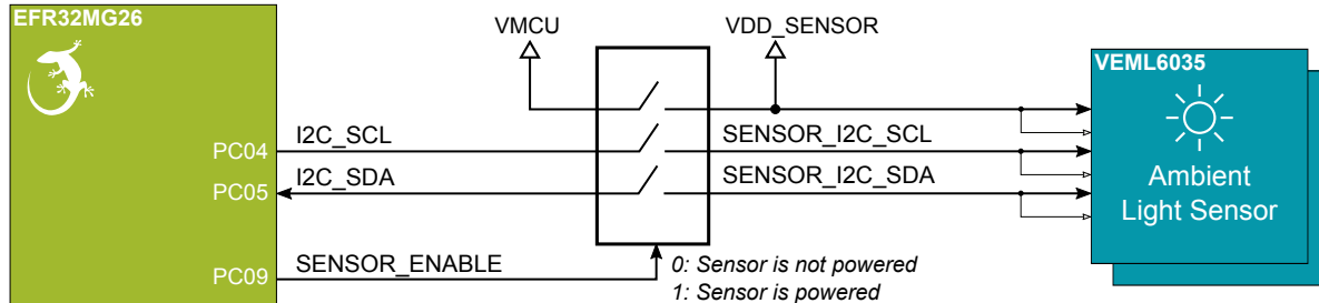
Figure 3.9. VEML6035 Ambient Light Sensor
