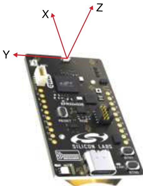
Figure 5.3. DUT Reference Planes
