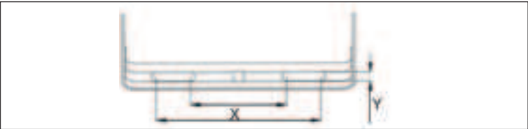
Fig. 5: Borehole distance
