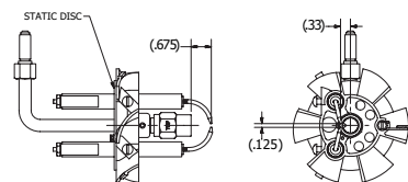
GUN ASSEMBLY
