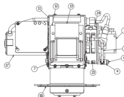
GUN ASSEMBLY
