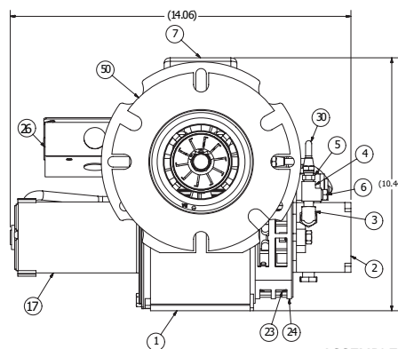
ASSEMBLED VIEWS
