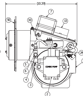
ASSEMBLED VIEWS
