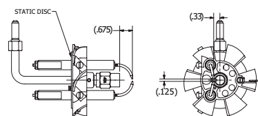
GUN ASSEMBLY
