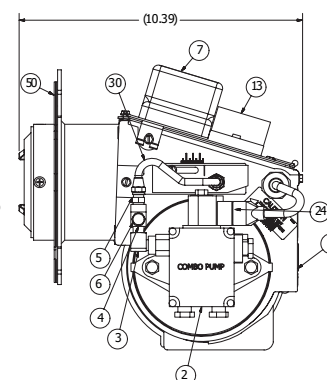
ASSEMBLED VIEWS
