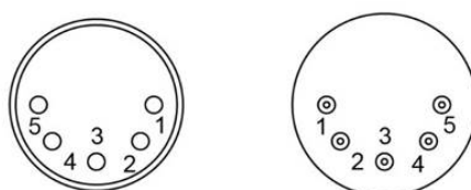
5 Pin XLR
