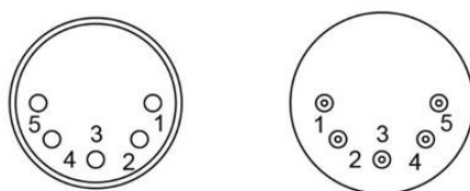
5 Pin XLR
