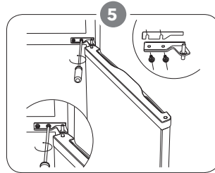
Unscrew the middle hinge and then lift the bottom door and put it on a soft pad to avoid scratch.
