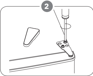
Unscrew the top hinge with a philips screw driver.
