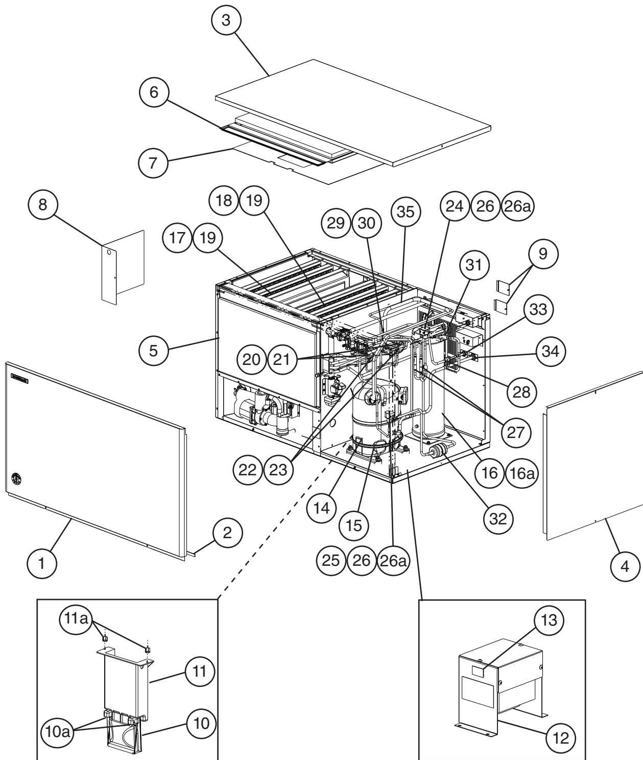
Main Transformer Box Assembly KM-1601SRJ(Z)3
