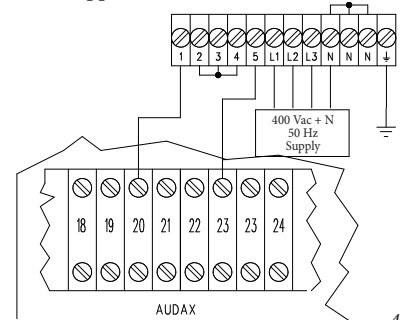
Supplementary Resistance configuration 6kW supplied with 400 Vac + N 50 Hz
