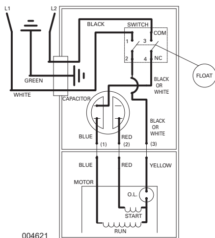
WIRING DIAGRAM FOR MODELS "M267", "D267", and "H267"
