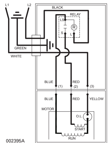
WIRING DIAGRAM FOR MODELS "M267-F", "E267-F", and "I267-F" 10/92 thru 04/18
