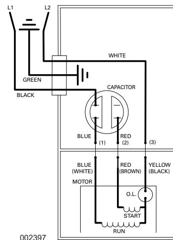
WIRING DIAGRAM FOR MODELS "N267", "E267", and "I267"
