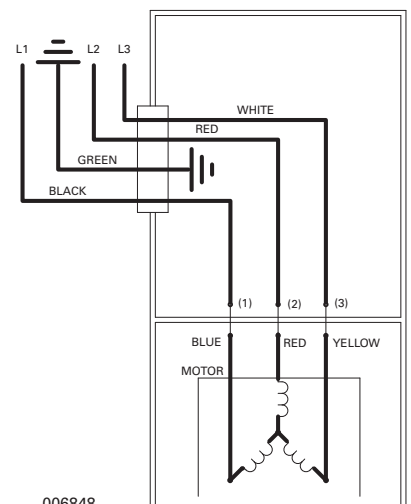
WIRING DIAGRAM FOR MODELS "J267-F", "F267-F" and "G267-F" 10/92 thru 12/18
