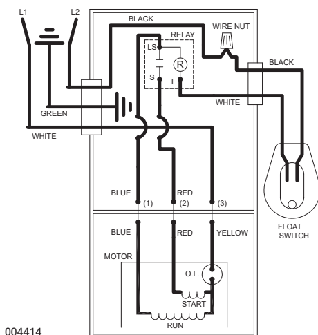
WIRING DIAGRAM FOR MODELS "WM267-C", "WM267-D" 10/92 thru 02/08
