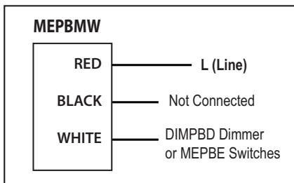
Figure 3: Button Only Operation (NO LED Indicator)
