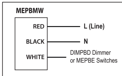
Figure 1: LED Indicator always ON
