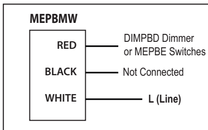
Figure 4: Button Only Operation (NO LED Indicator)
