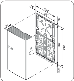
Montage mural (inclus)
