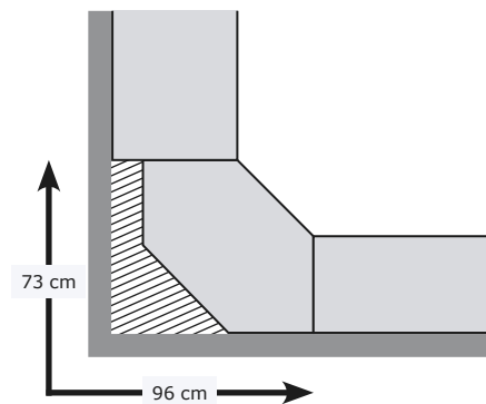
Corner section with one 35 cm deep frame and one 58 cm deep frame.
