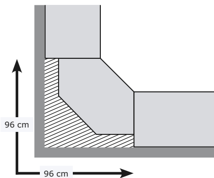
Corner section with two 58 cm deep frames.
