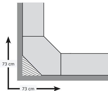
Corner section with two 35 cm deep frames.
