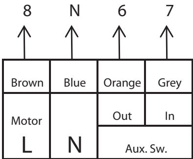
HP22 2 Port Valve (Hot Water)
