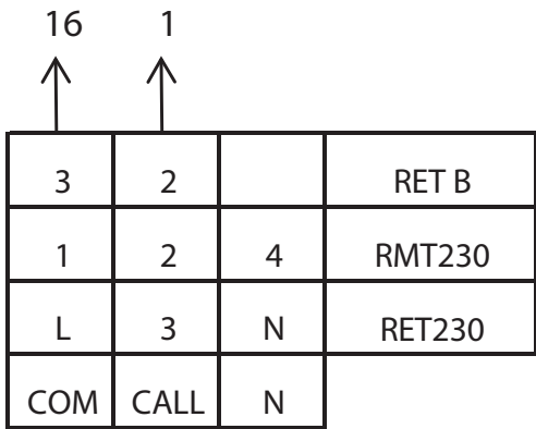
Room Thermostat - Zone 2
