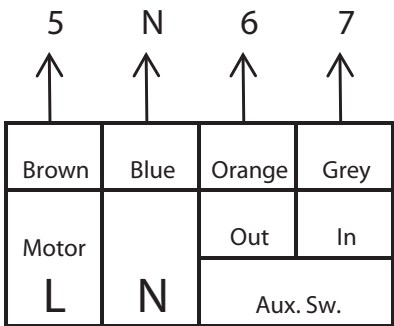
HP22 2 Port Valve (Heating Zone 2)
