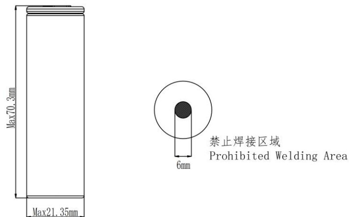
图 1. 电芯尺寸(含套膜) Figure 1. Cell dimension with tube.
