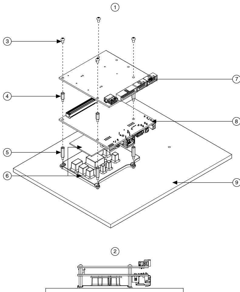
Figure 7. Mounting on a Panel or Plate with Conduction Path
