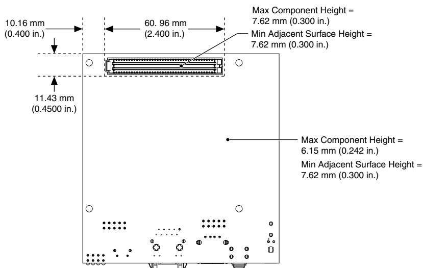
Figure 6. Maximum Component Height of Secondary Side
