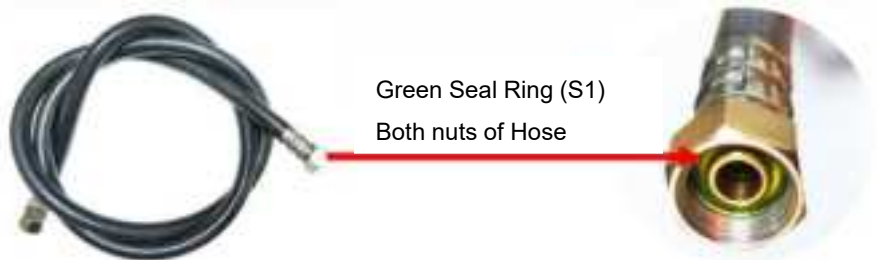
Green Seal Ring S1: 8x13x2
