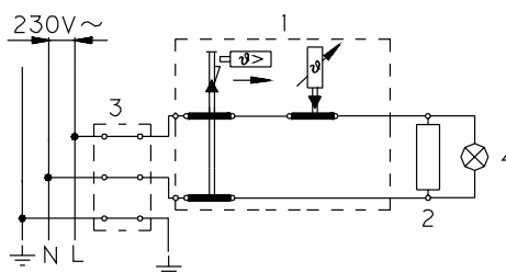
Electric installation
