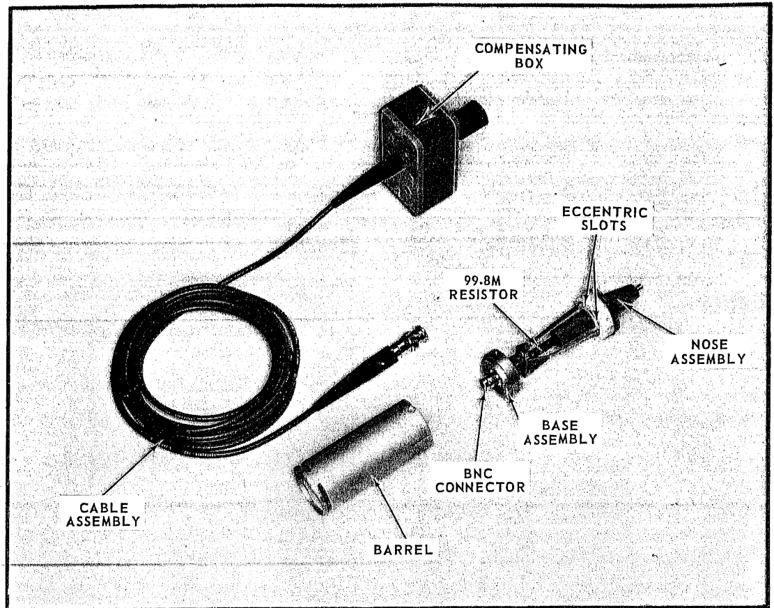
Fig. 3. Probe Assembly.
